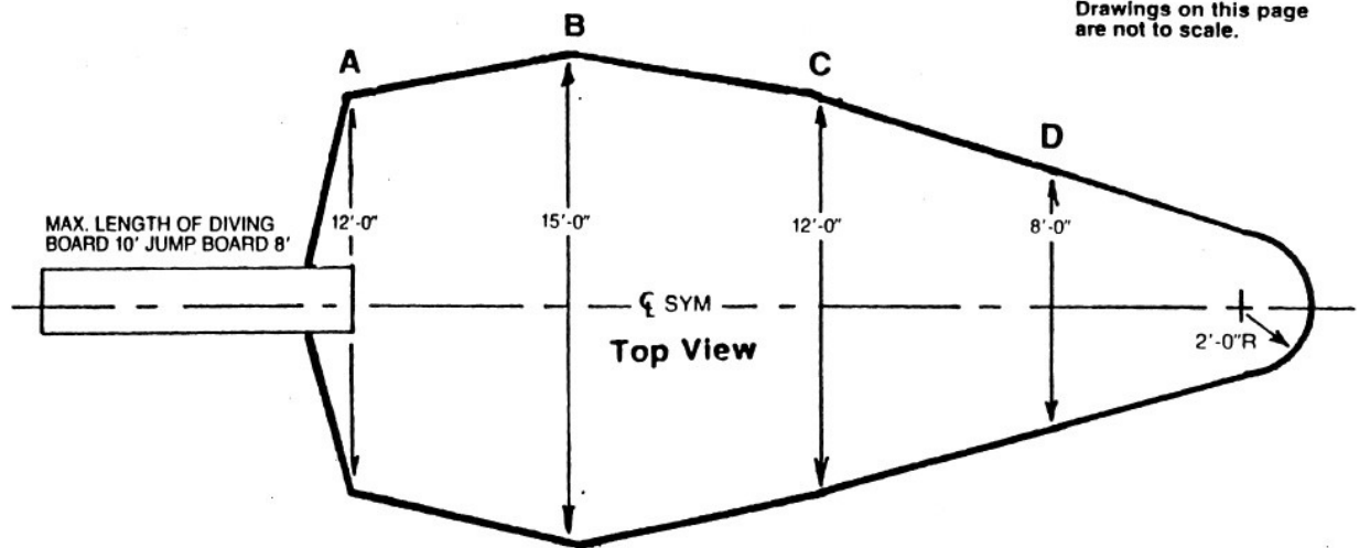
FIGURE R326.10(7)
