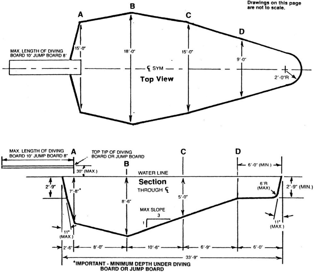
MINIMUM DIMENSIONS FOR A TYPE IV POOL
