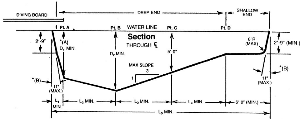
FIGURE R326.10(1) MINIMUM DIMENSIONS FOR RESIDENTIAL POOLS WITH DIVING EQUIPMENT (LONGITUDINAL CROSS-SECTION AT CENTERLINE)
